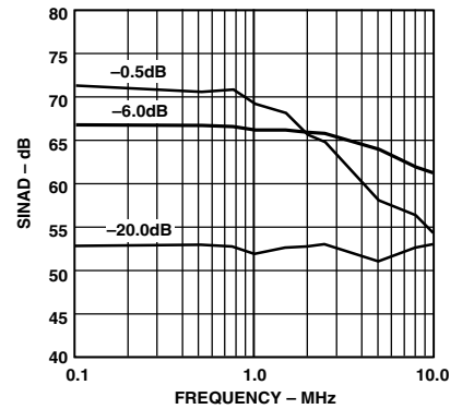
TPC 24. SINAD vs. Input Frequency (Input Span = 5.0 V p-p, V CM = 2.5 V)
