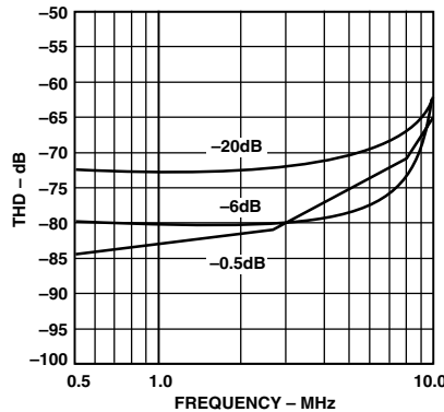
TPC 23. THD vs. Input Frequency (Input Span = 2.0 V p-p, V CM = 2.5 V)
