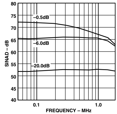
TPC 6. SINAD vs. Input Frequency (Input Span = 5.0 V p-p, V CM = 2.5 V)
