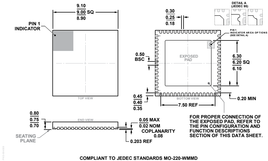
Figure 44. 64-Lead Lead Frame Chip Scale Package [LFCSP] 9 mm x 9 mm and 0.75 mm Package Height (CP-64-17) Dimensions shown in millimeters
