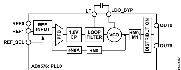
Figure 23. PLL0 Loop Configuration 1
