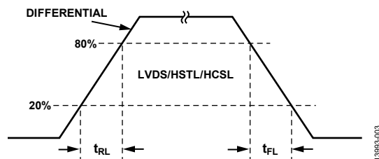
Figure 3. LVDS, HSTL, and HCSL Timing, Differential
