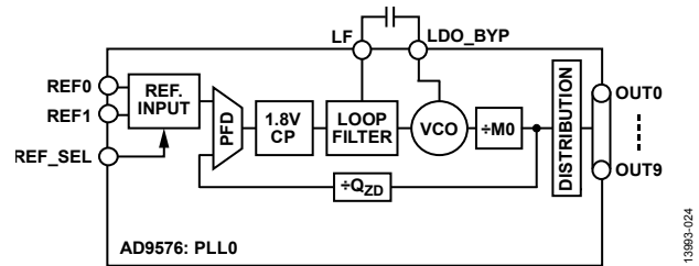
Figure 24. PLL0 Loop Configuration 2
