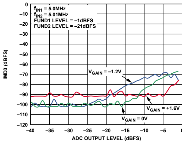
Figure 29. IMD3 vs. ADC Output Level
