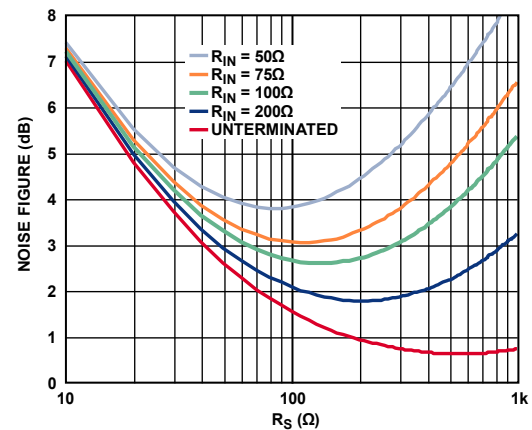
Figure 36. Noise Figure vs. R_S for Various Fixed Values of R_{IN} , Active Termination Matched Inputs, V_{GAIN} = 1.6 \text{ V}
