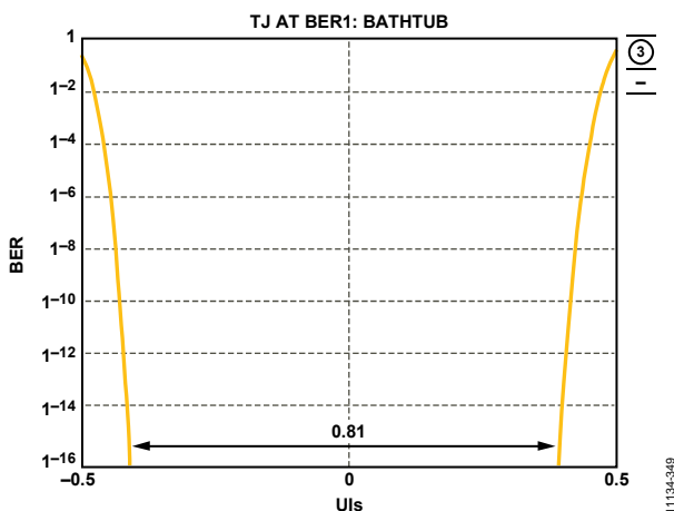
Figure 51. Digital Outputs Bathtub, External 100 Ω Terminations at 2.5 Gbps
