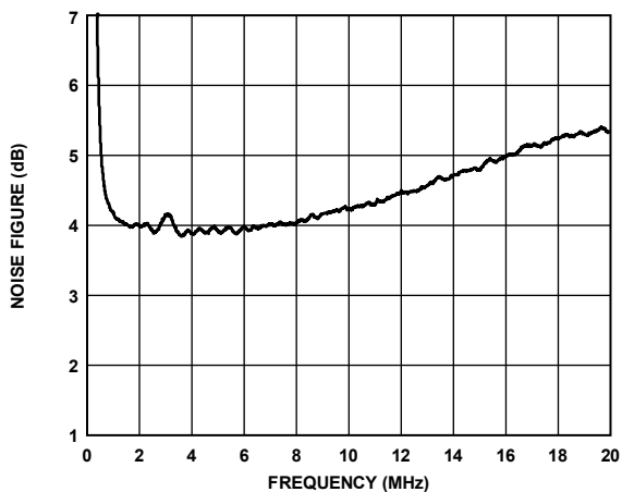
Figure 30. Noise Figure vs. Frequency R_S = R_{IN} = 100\Omega , LNA Gain = 17.9 dB, PGA Gain = 30 dB, V_{GAIN} = 1.6V
