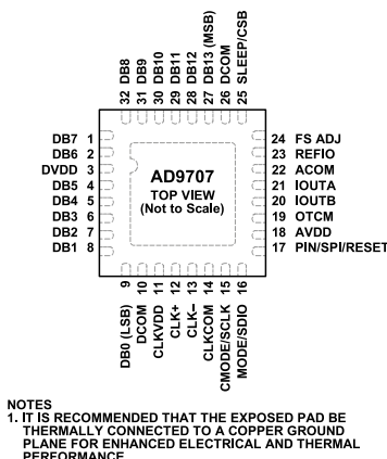
Figure 3. AD9707 Pin Configuration
