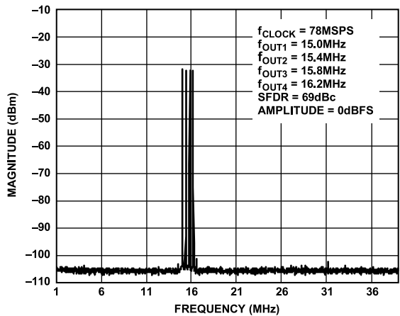
Figure 43. Four-Tone SFDR
