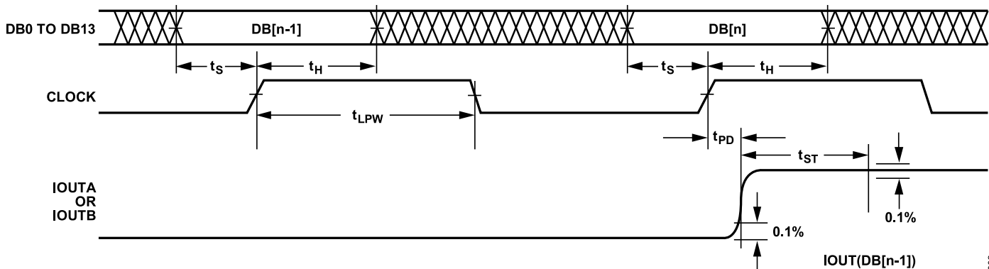
Figure 2. Parallel Data Interface Timing Diagram
