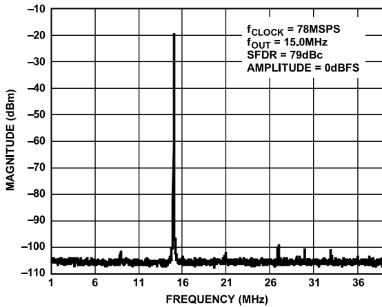
Figure 41. Single-Tone SFDR
