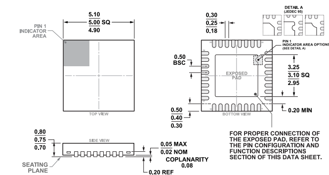
Figure 91. 32-Lead Lead Frame Chip Scale Package [LFCSP] 5 mm x 5 mm Body and 0.75 mm Package Height (CP-32-7) Dimensions shown in millimeters
