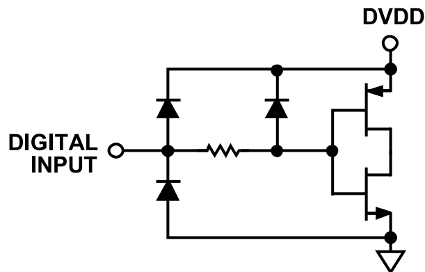
Figure 79. Equivalent Digital Input
