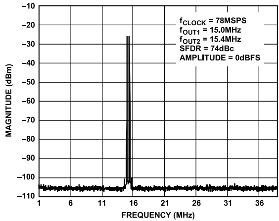
Figure 42. Dual-Tone SFDR
