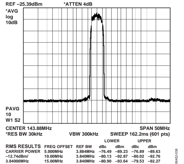
Figure 41. AD9778A ACLR, f_{DATA} = 122.88 MSPS, 4x Interpolation, f_{DAC}/4 Modulation
