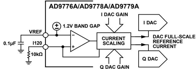
Figure 76. Reference Circuitry
