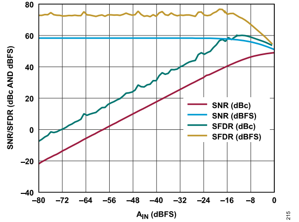
Figure 51. Single-Tone SFDR and SNR vs. A_{IN} at f_{IN} = 5400 MHz, f_S = 4 GSPS
