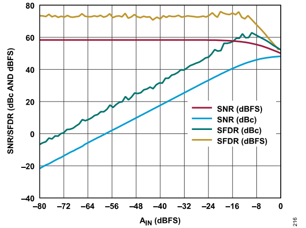
Figure 52. Single-Tone SFDR and SNR vs. A_{IN} at f_{IN} = 6300 MHz, f_S = 4 GSPS
