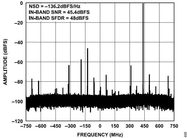
Figure 50. Single-Tone FFT at f_{IN} = 7200 MHz
