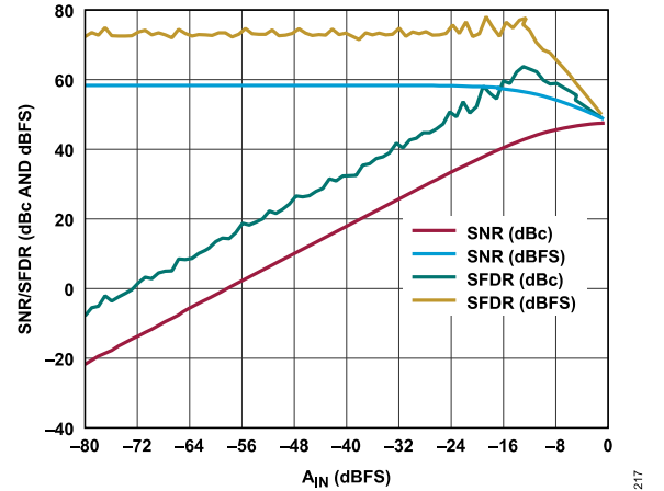
Figure 53. Single-Tone SFDR and SNR vs. A_{IN} at f_{IN} = 7200 MHz, f_S = 4 GSPS
