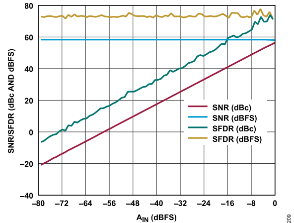
Figure 39. Single-Tone SFDR and SNR vs. A_{IN} at f_{IN} = 450 MHz, f_S = 4 GSPS
