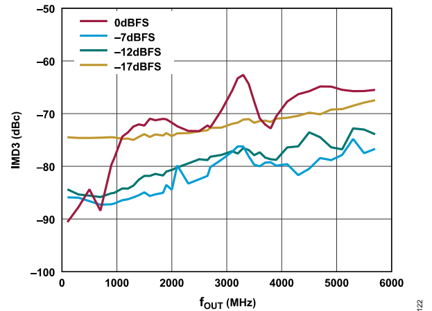
Figure 22. IMD3 vs. f_{OUT} over Digital Scale, 12 GSPS DAC Sample Rate, Channel Interpolation 4 \times , Main Interpolation 8 \times , Mode 16B; IMD3 is a Two-Tone Test, and the Scale per Tone is 6 dB Lower than the Reported Digital Scale
