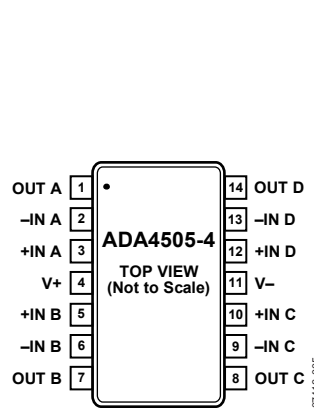
Figure 5. 14-Lead TSSOP (RU-14)
