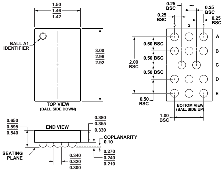
COMPLIANT TO JEDEC STANDARDS MO-153-AB-1 Figure 64. 14-Ball Wafer Level Chip Scale Package [WLCSP] (CB-14-1) Dimensions shown in millimeters
