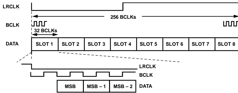
Figure 50. TDM Mode
