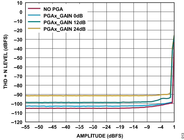
Figure 13. THD + N Level vs. Amplitude, f_s = 48 kHz, Signal Path = AINx to SDATA0, No PGA and PGA Gain Settings (0 dB, 12 dB, 24 dB), ADC0 and ADC1 Differential Mode
