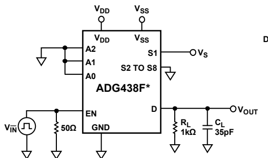
Figure 27. Enable Delay, t_{\text{ON}}(\text{EN}) , t_{\text{OFF}}(\text{EN})
