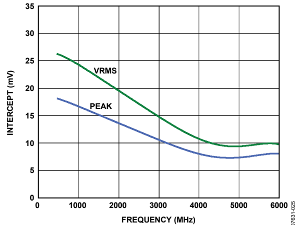
Figure 25. VRMS and PEAK Intercept vs. Frequency, Supply 3 V
