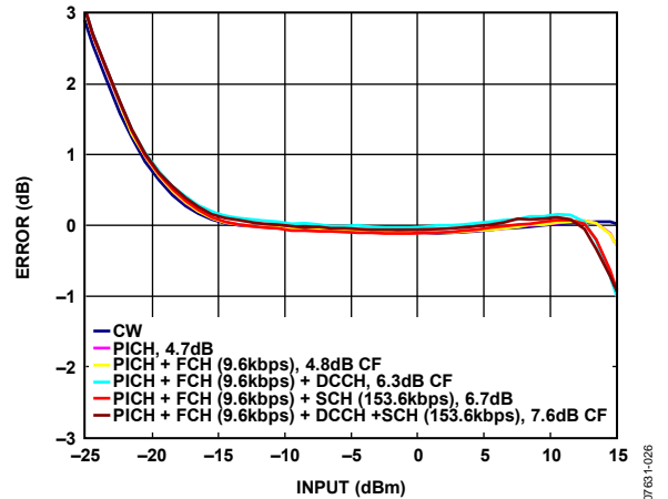
Figure 26. Error from CW Linear Reference vs. Input with Various CDMA2000 Reverse Link Waveforms at 1900 MHz, C_{FLTR} = 10 nF, C_{OUT} = Open
