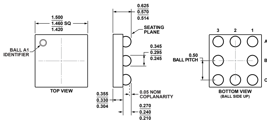
Figure 68. 8-Ball Wafer Level Chip Scale Package [WLCSP] (CB-8-3)
