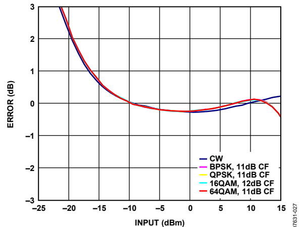
Figure 27. Error from CW Linear Reference vs. Input with Various 802.16 OFDM Waveforms at 3500 MHz, 10 MHz Signal BW, and 256 Subcarriers for All Modulated Signals, C_{FLTR} = 10 nF, C_{OUT} = Open
