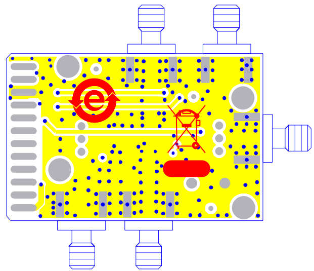
Figure 67. Layout of Evaluation Board, Circuit Side
