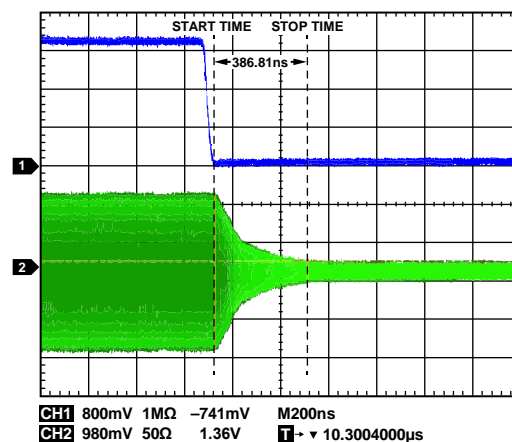
Figure 28. VVA Gain Settling Time, Minimum to Maximum VVA Attenuation
