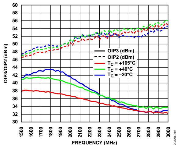
Figure 16. OIP3/OIP2 vs. Frequency for Various Temperatures
