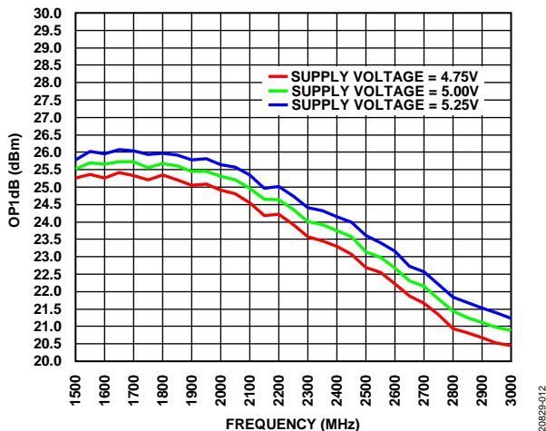
Figure 12. OP1dB vs. Frequency for Various Supplies
