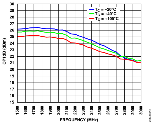
Figure 13. OP1dB vs. Frequency for Various Temperatures
