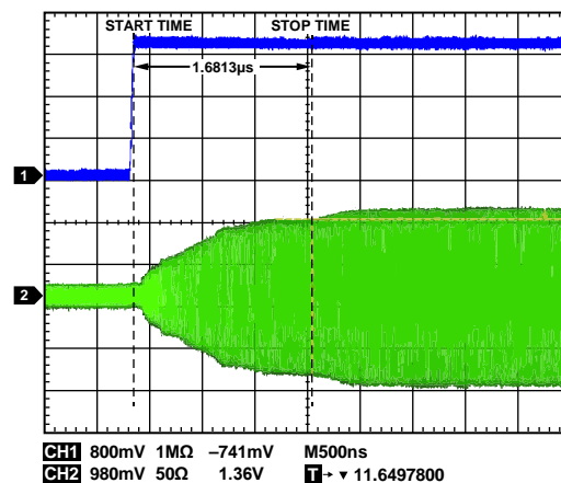
Figure 29. VVA Gain Settling Time, Maximum to Minimum VVA Attenuation
