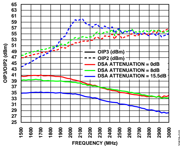
Figure 15. OIP3/OIP2 vs. Frequency at Various DSA Values, VVA Attenuation = 0 dB
