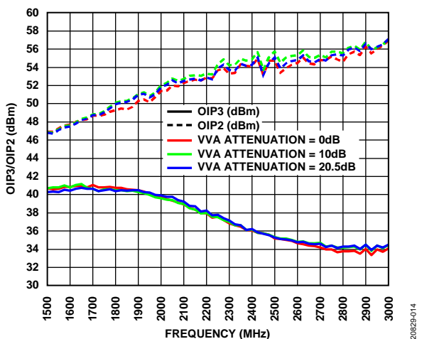
Figure 14. OIP3/OIP2 vs. Frequency at Various VVA Attenuation Values, DSA Attenuation = 0 dB
