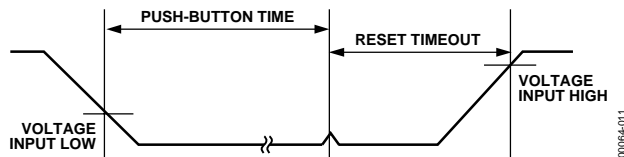
Figure 12. Push-Button Reset Timing Diagram
