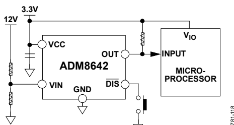
Figure 18. ADM8642 Typical Application Circuit
