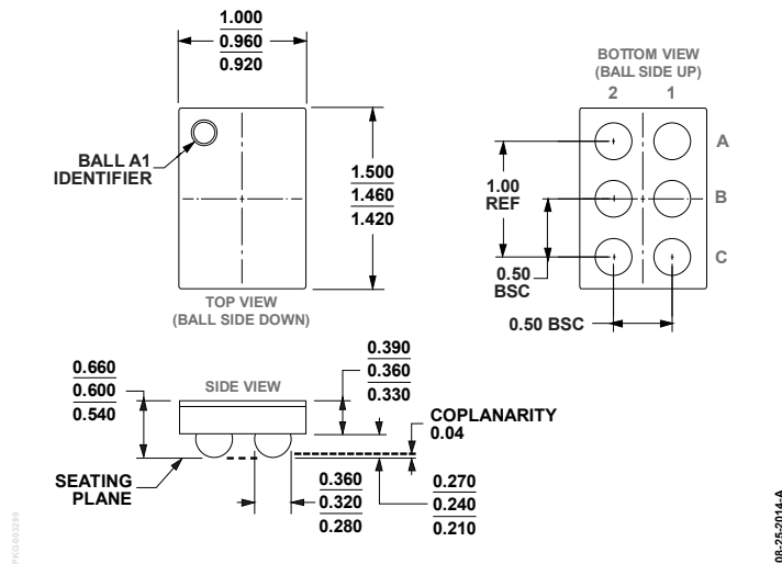
Figure 22. 6-Ball Wafer Level Chip Scale Package [WLCSP] (CB-6-17) Dimensions shown in millimeters
