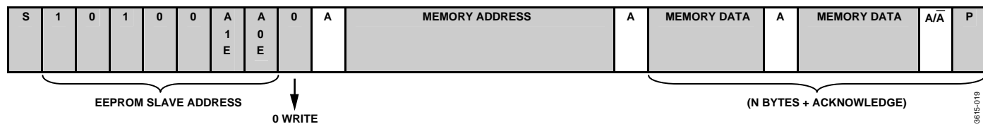
Figure 19. EEPROM Write
