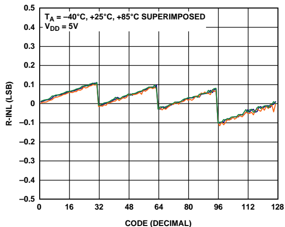
Figure 10. R-INL—7-Bit RDAC
