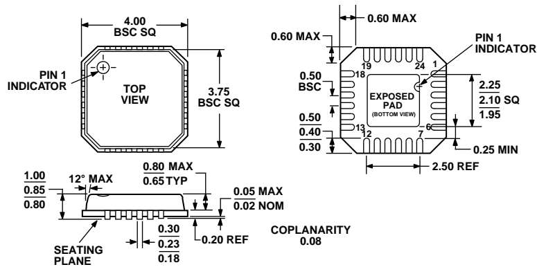
Figure 34. 24-Lead Lead Frame Chip Scale Package [LFCSP_VQ]
