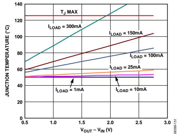
Figure 41. Junction Temperature vs. Power Dissipation, 500 mm 2 of PCB Copper, T_A = 50^\circ\text{C}
