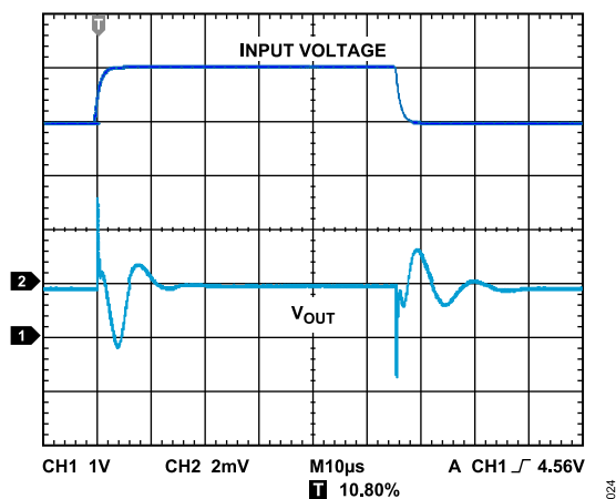
Figure 26. Line Transient Response, C_{IN} = C_{OUT} = 1 \mu\text{F} , I_{LOAD} = 1 \text{ mA}
