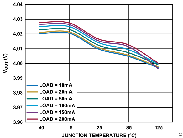
Figure 34. 4 V LDO Circuit, Typical Load Regulation over Temperature
