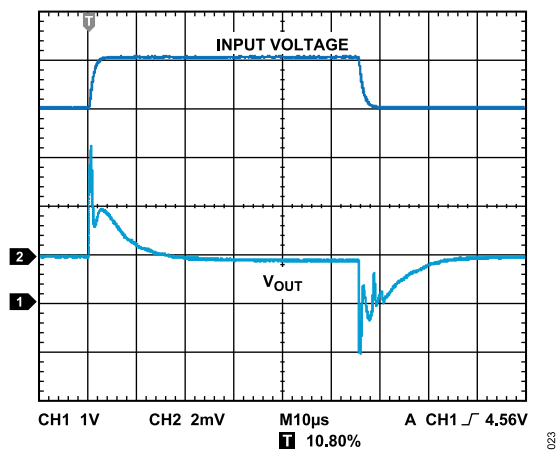
Figure 25. Line Transient Response, C_{IN} = C_{OUT} = 1 \mu\text{F} , I_{LOAD} = 200 \text{ mA}
