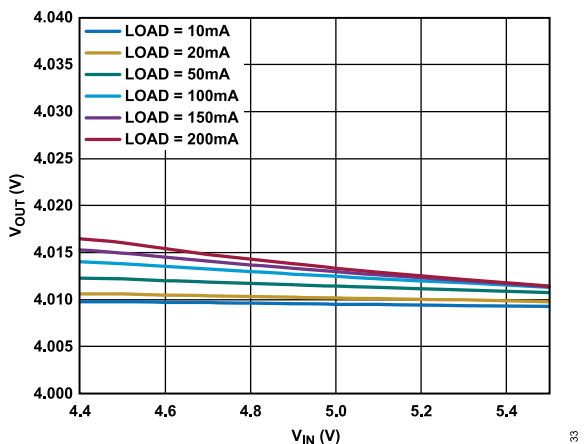
Figure 35. 4 V LDO Circuit, Typical Line Regulation over Load Current
