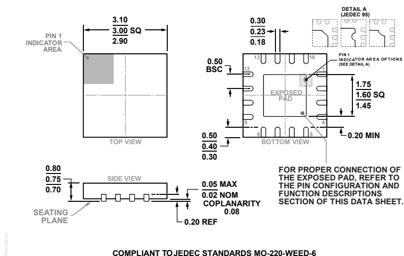
COMPLIANT TO JEDEC STANDARDS MO-220-WEED-6 Figure 47. 16-Lead Lead Frame Chip Scale Package [LFCSP] 3 mm × 3 mm Body and 0.75 mm Package Height (CP-16-22) Dimensions shown in millimeters
