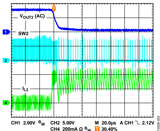
Figure 53. Output Short
