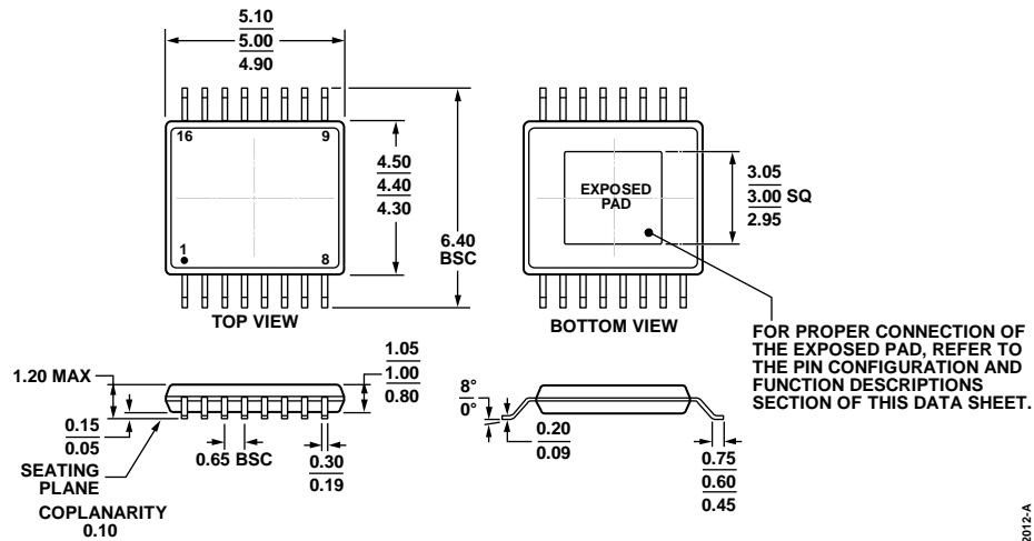
Figure 60. 16-Lead Thin Shrink Small Outline With Exposed Pad [TSSOP_EP] (RE-16-2)
