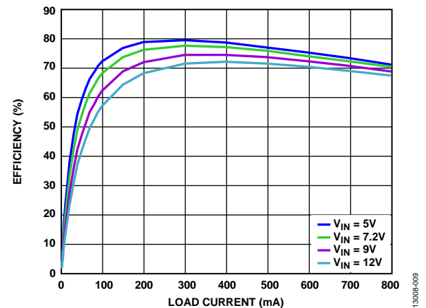
Figure 9. Channel 1 PWM Efficiency vs. Load Current, V_{OUT1} = 1.2\text{ V}
