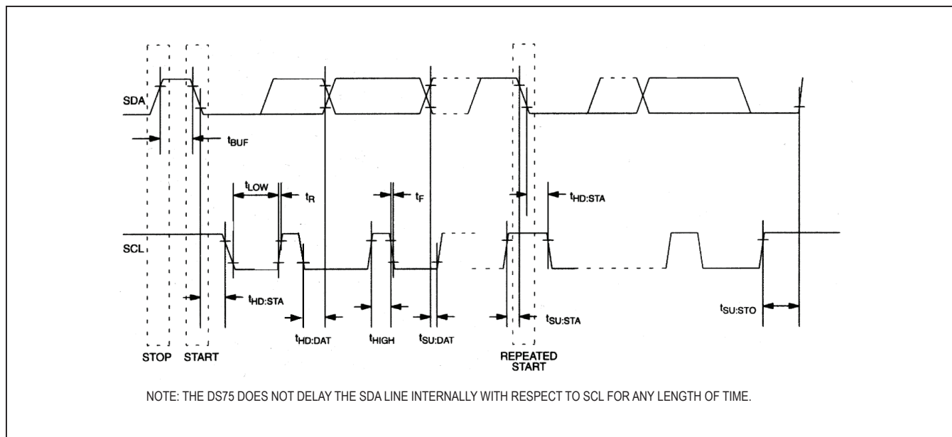
Figure 2. Timing Diagram
