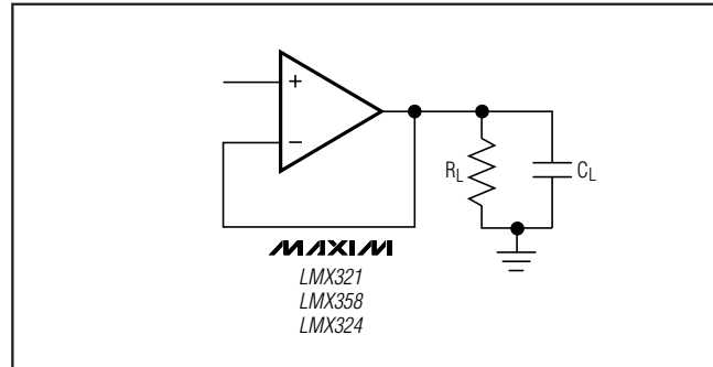
Figure 3. Capacitive-Load-Driving Circuit
