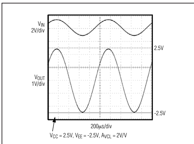
Figure 2. Rail-to-Rail Output Swing
