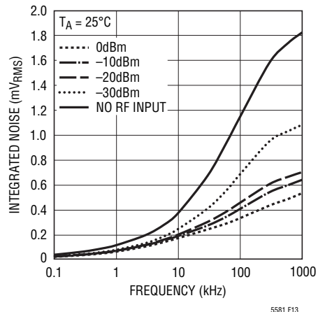
Figure 13. Integrated Output Voltage Noise
