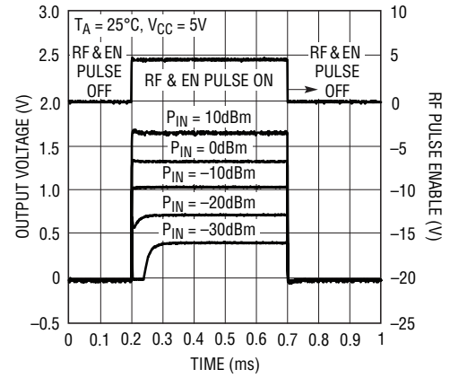
Output Transient Response with RF and EN Pulse
