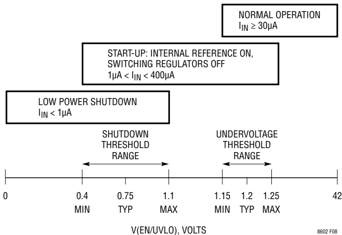
Figure 8. EN/UVLO Thresholds
