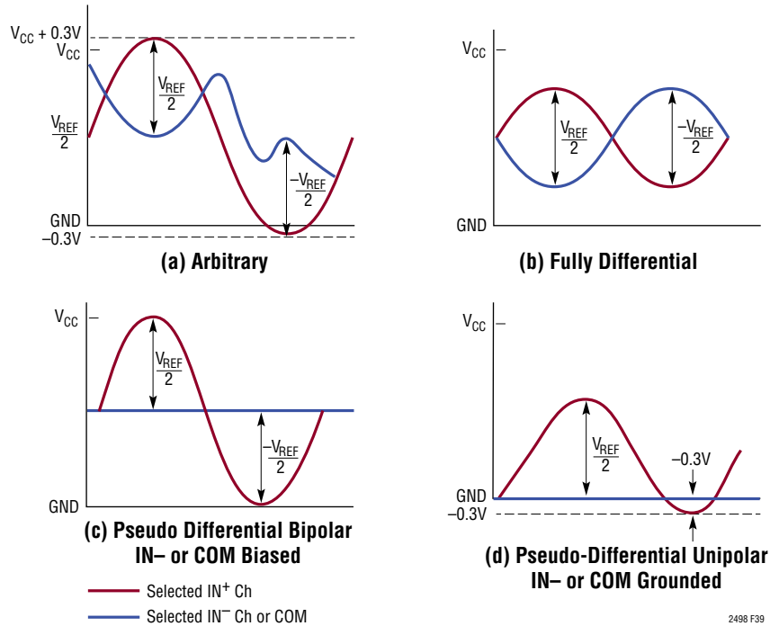
Figure 39. Input Range
