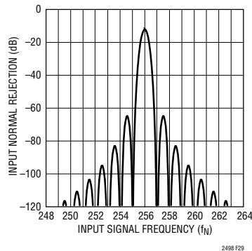
Figure 29. Input Normal Mode Rejection 2x Speed Mode
