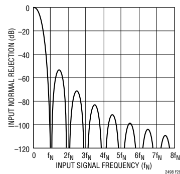
Figure 28. Input Normal Mode Rejection 2x Speed Mode
