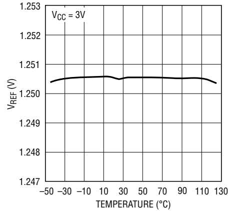
REFOUT Voltage vs Temperature
