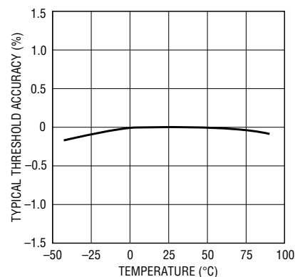
Figure 4. LTC2903 Typical Threshold Accuracy vs Temperature
