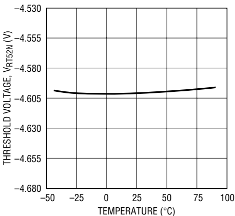
-5.2V Threshold Voltage vs Temperature
