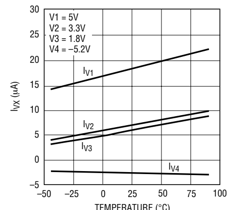
Supply Currents vs Temperature (LTC2903-C1)
