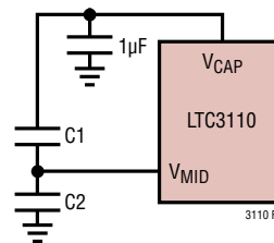
Figure 8. V_{MID} Charge Balancer Output
