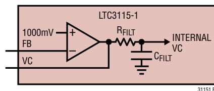
Figure 11. Internal Loop Filter
