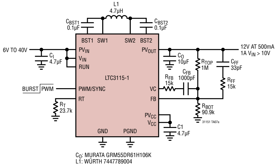
Miniature Size 1.5MHz 12V Supply
