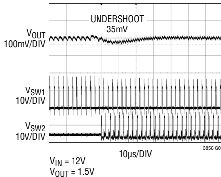
Stage Shedding Transition, 1-Phase to 2-Phase
