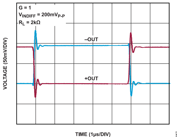
Figure 56. Small Signal Step Response
