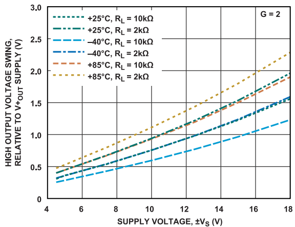
Figure 62. High Output Voltage Swing vs. Supply Voltage
