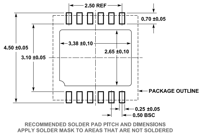
Figure 106. 12-Lead 4 mm × 4 mm DFN (05-08-1791)
