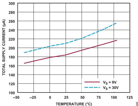
Figure 44. Shutdown Supply Current vs. Temperature
