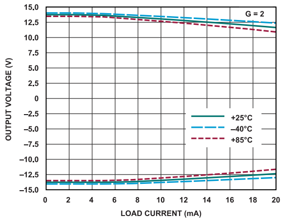
Figure 60. Output Voltage Swing vs. Load Current
