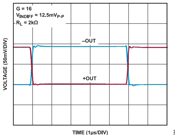
Figure 55. Small Signal Step Response
