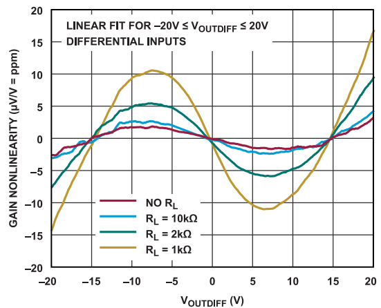
Figure 19. Differential Gain Nonlinearity vs. Output Voltage
