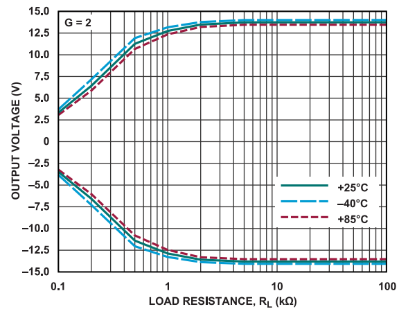
Figure 61. Output Voltage Swing vs. Load Resistance
