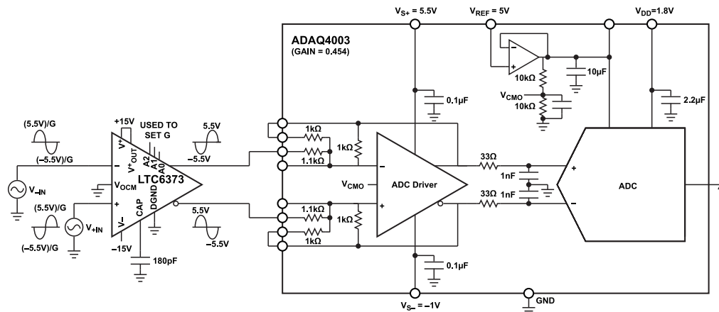
Figure 93. LTC6373 Driving ADAQ4003 (Gain = 0.454)
