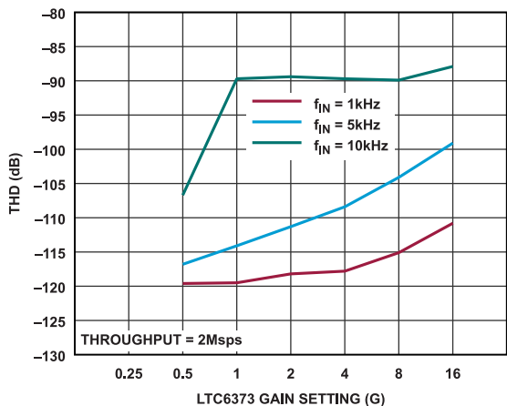
Figure 95. THD for LTC6373 Driving ADAQ4003 (Gain = 0.454)
