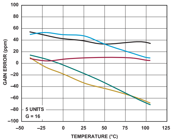
Figure 20. Differential Gain Error vs. Temperature
