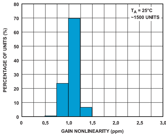
Figure 18. Typical Distribution of Differential Gain Nonlinearity
