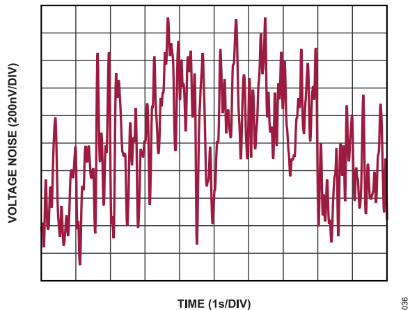
Figure 35. Input Referred 0.1 Hz to 10 Hz Voltage Noise (G = 1)
