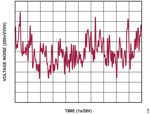
Figure 33. Input Referred 0.1 Hz to 10 Hz Voltage Noise (G = 4)
