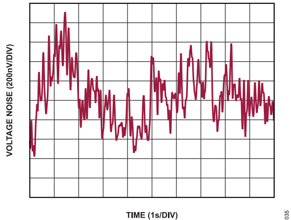
Figure 34. Input Referred 0.1 Hz to 10 Hz Voltage Noise (G = 2)
