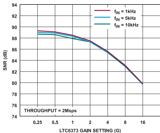
Figure 97. SNR for LTC6373 Driving ADAQ4003 (Gain = 0.9)
