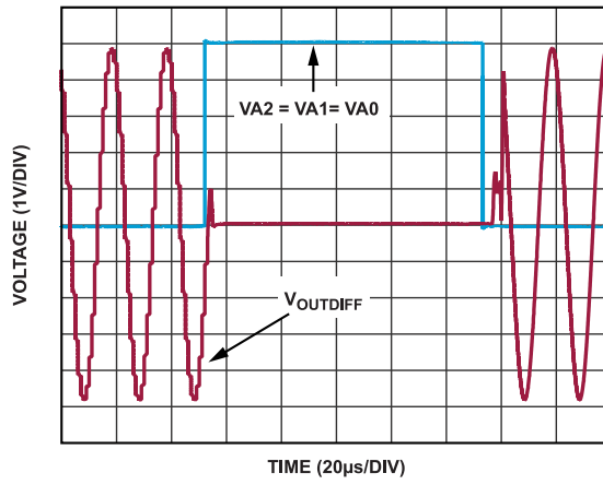
Figure 73. Turn-On and Turn-Off Transient Response
