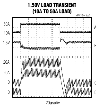
A. LOAD CURRENT, ( I_{LOAD} = 10A TO 50A ), 50A/div B. OUTPUT VOLTAGE (1.50V NO LOAD), 100mV/div C. I_{L1} , 10A/div D. I_{L2} , 10A/div
