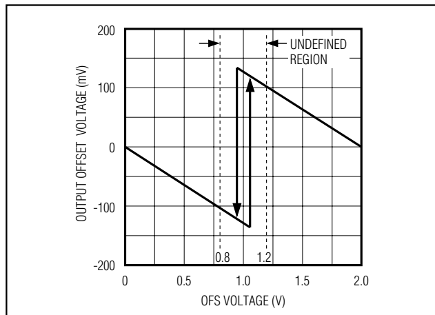
Figure 6. Offset Voltage
