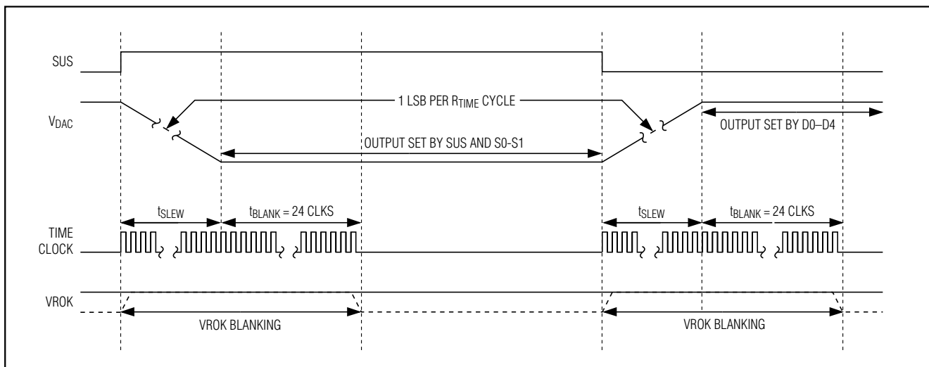
Figure 4. Suspend Transition
