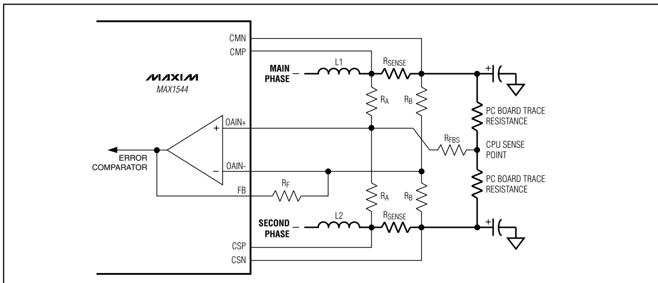
Figure 10. Voltage-Positioning Gain
