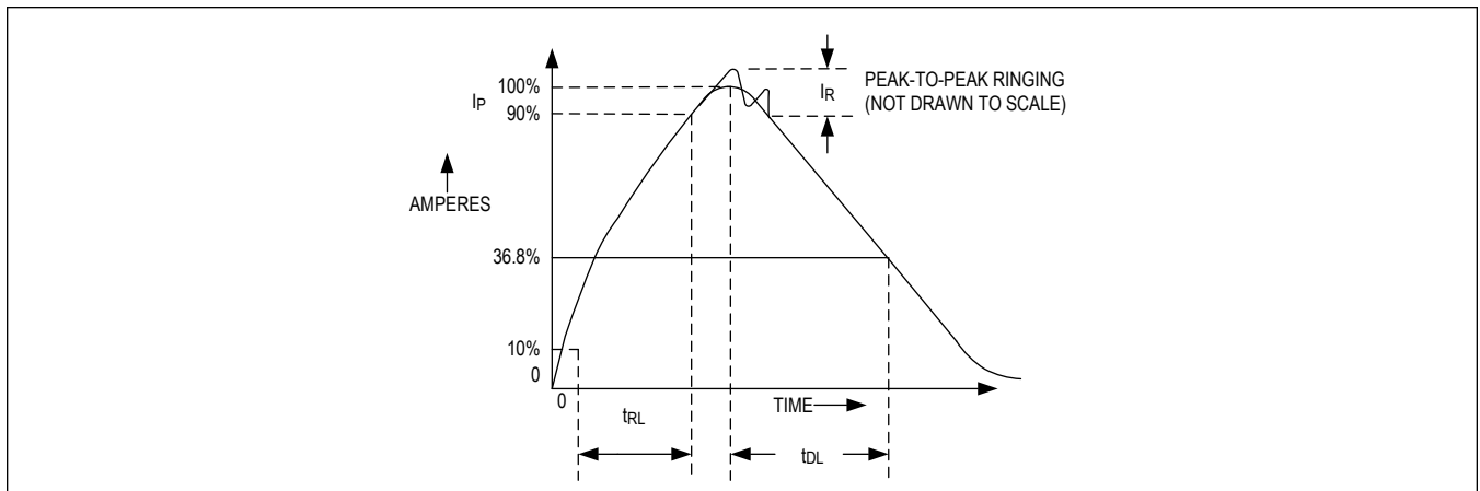
Figure 7. Human Body Current Waveform
