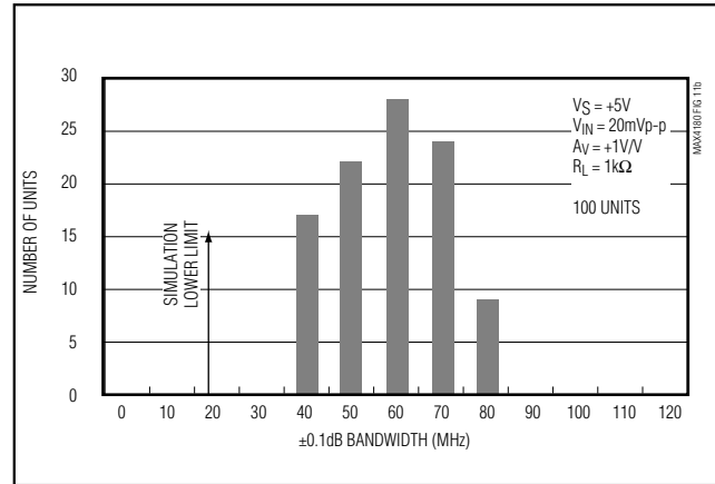
Figure 11b. MAX4181 \pm 0.1dB Bandwidth Distribution (Single Supply)
