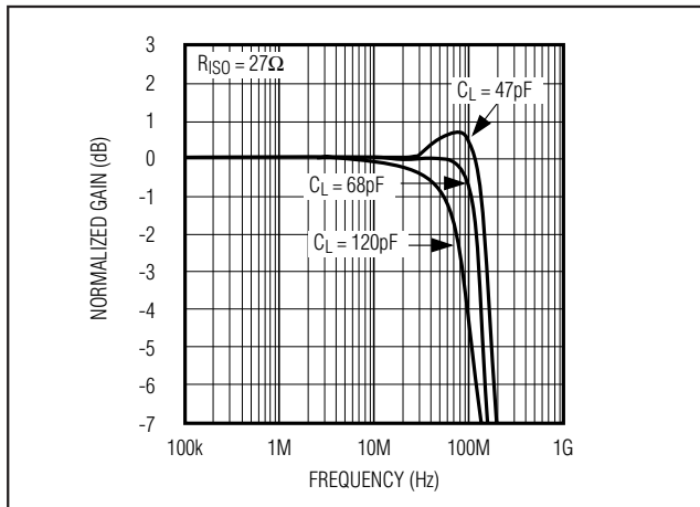
Figure 9. Small-Signal Gain vs. Frequency with Load Capacitance and 27\Omega Isolation Resistor
