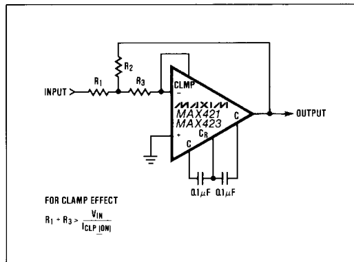
Figure 4. Inverting Amplifier with Optional Clamp.
