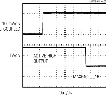
PROPAGATION DELAY V_{CC} RISING
