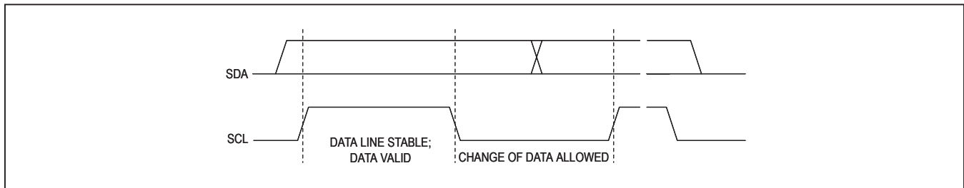
Figure 4. Bit Transfer
