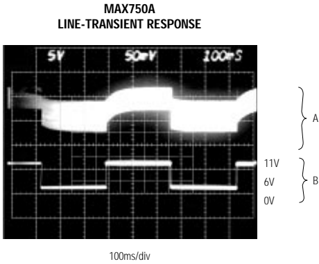
A: V_{OUT} , 50mV/div, AC-COUPLED B: V_+ , 5V/div, 6.0V TO 11.0V I_{OUT} = 300mA
