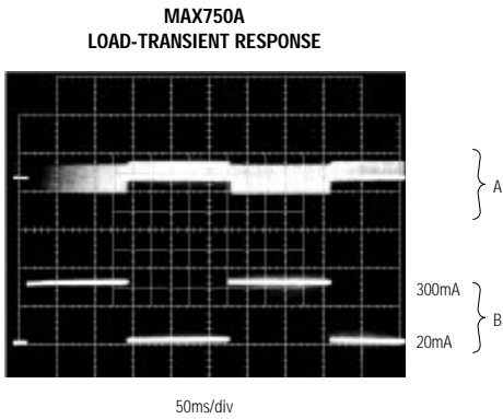
A: V_{OUT} , 50mV/div, AC-COUPLED B: I_{OUT} , 200mA/div, 20mA TO 300mA V_+ = 9V
