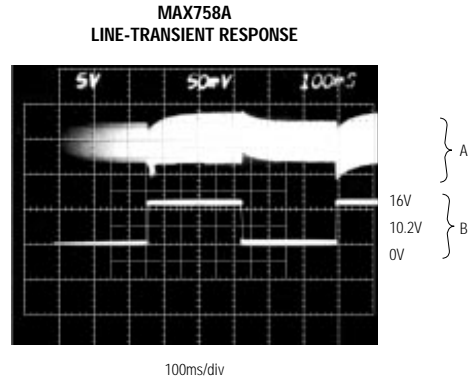
A: V_{OUT} , 50mV/div, AC-COUPLED B: V_+ , 5V/div, 10.2V TO 16.0V I_{OUT} = 750mA
