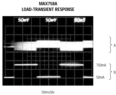
A: V_{OUT} , 50mV/div, AC-COUPLED B: I_{OUT} , 500mA/div, 50mA TO 750mA V_+ = 12V
