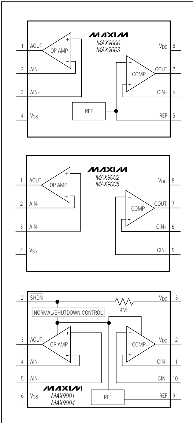
Figure 1. MAX9000–MAX9005 Functional Diagrams
