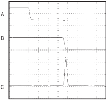
100ns/div A = IN+, 100mV/div B = OUT, 5V/div C = ICC, 1mA/div
