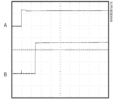
5ms/div A = VCC, 2V/div B = OUT, 1V/div
