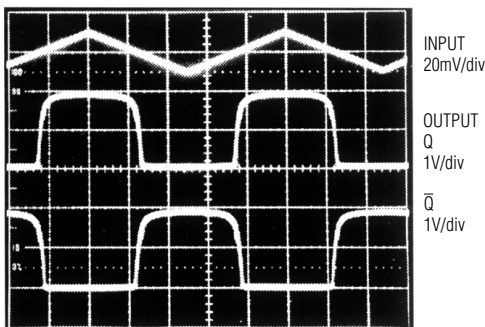
MAX912/MAX913 RESPONSE
