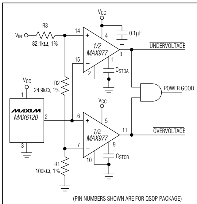
Figure 5. Window Comparator
