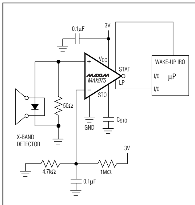
Figure 6. Toll-Tag Reader
