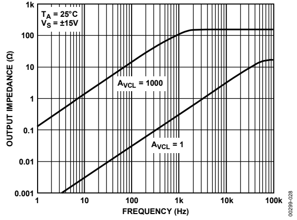
Figure 28. Closed-Loop Output Resistance vs. Frequency
