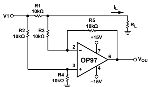
Figure 36. Current Monitor
