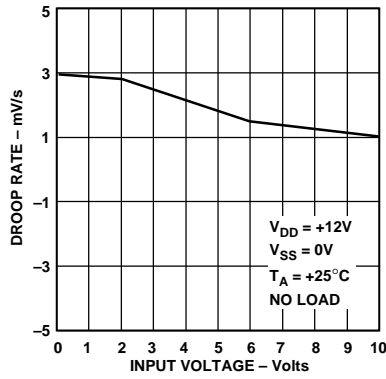
Droop Rate vs. Input Voltage
