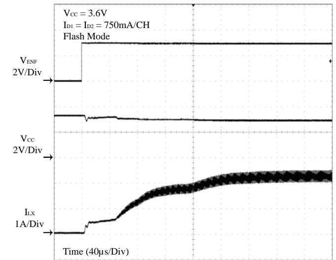
Figure 8 LX Current
