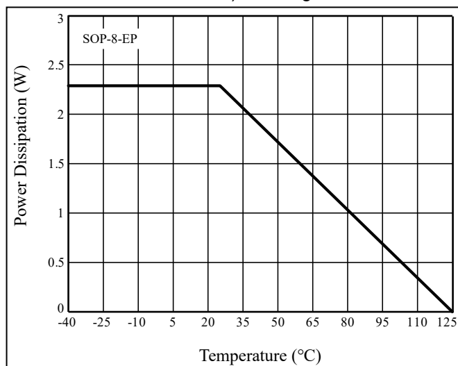
Figure 34 Dissipation Curve
