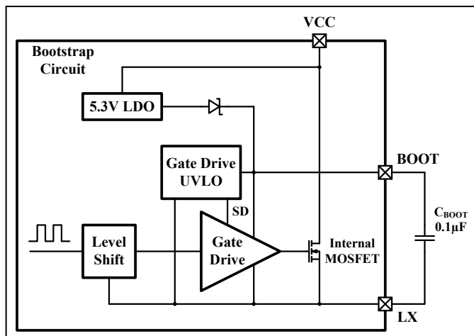
Figure 26 Bootstrap Circuit
