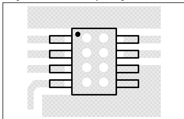
Figure 35 Board Via Layout For Thermal Dissipation
