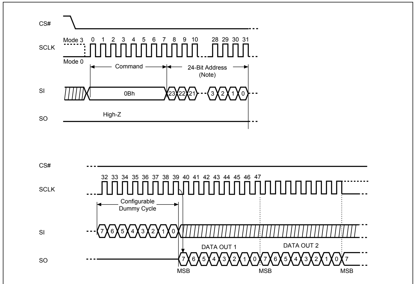
Figure 33. Read at Higher Speed (FAST_READ) Sequence (SPI Mode)
