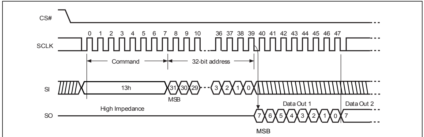
Figure 48. Read Data Bytes using 4 Byte Address Sequence (READ4B)
