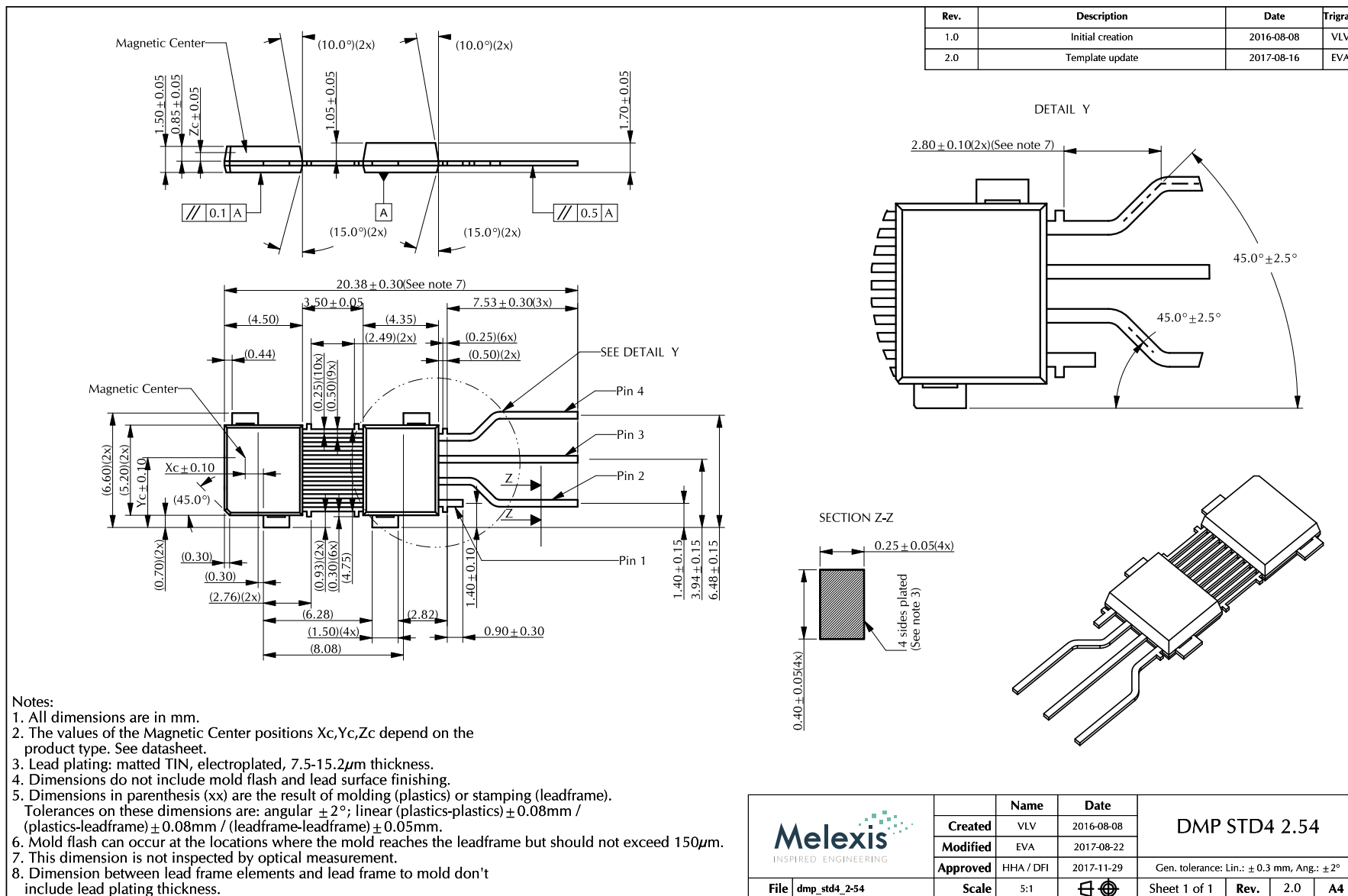
fig. 41 - DMP-4 STD4 2.54 Package Outline Drawing
