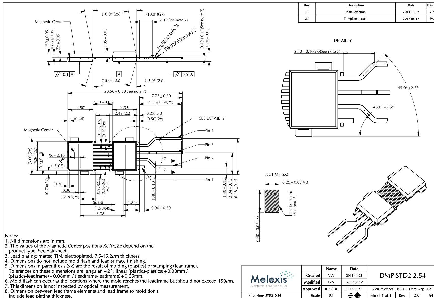
fig. 39 - DMP-4 STD2 2.54 Package Outline Drawing
