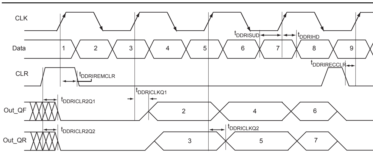
Figure 2-21 • Input DDR Timing Diagram
